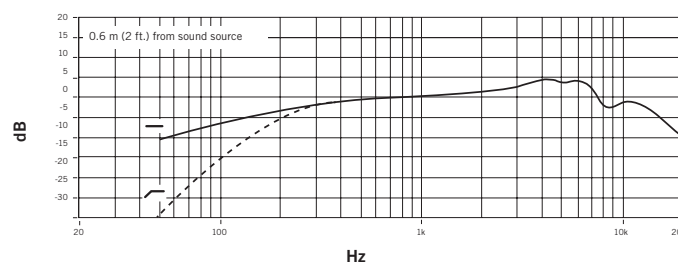
Frequency Response
